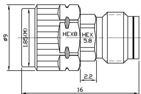
Drawing(mm)
