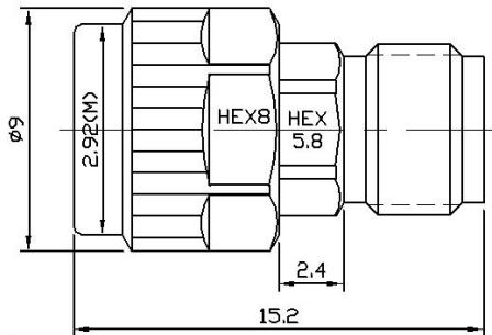
Drawing(mm)
