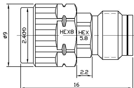
Drawing(mm)
