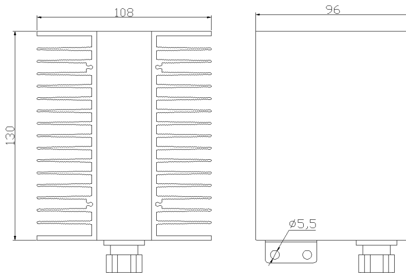
100W PIM Load
